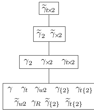
Fig. 2. The Hasse diagram representing the preorder \leq on the considered domination parameters.
