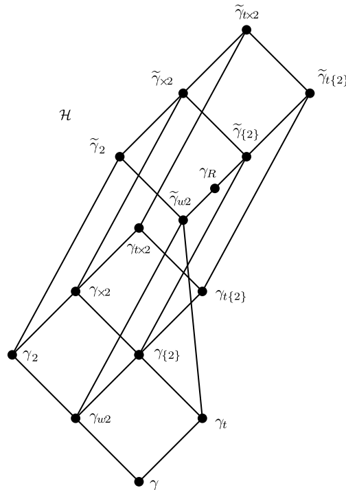
Fig. 1. Hasse diagram of the relation \leq among various domination parameters (see Section 3).
