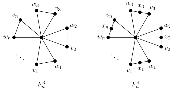
Fig. 3. Graphs F_n^3 and F_n^4 .
