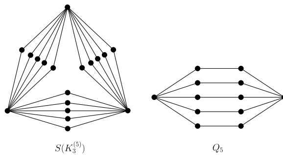
Fig. 5. Examples of graphs S(K_3^{(n)}) and Q_n .
