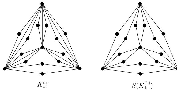
Fig. 4. Examples of graphs K_n^{**} and S(K_n^{(2)}) .
